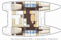
Plan version 4 cabines 4 B&B / 4 cabine version - 4 washrooms
